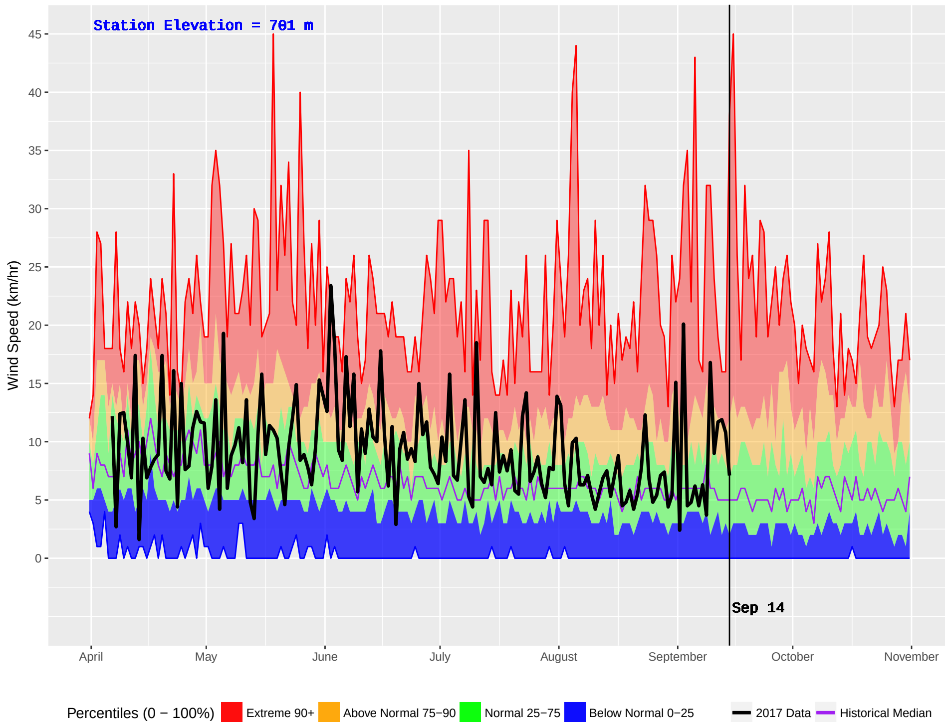
HORSEFLY (230) : Historical (1971–2016) and Current (2017) Noon Wind Speed
