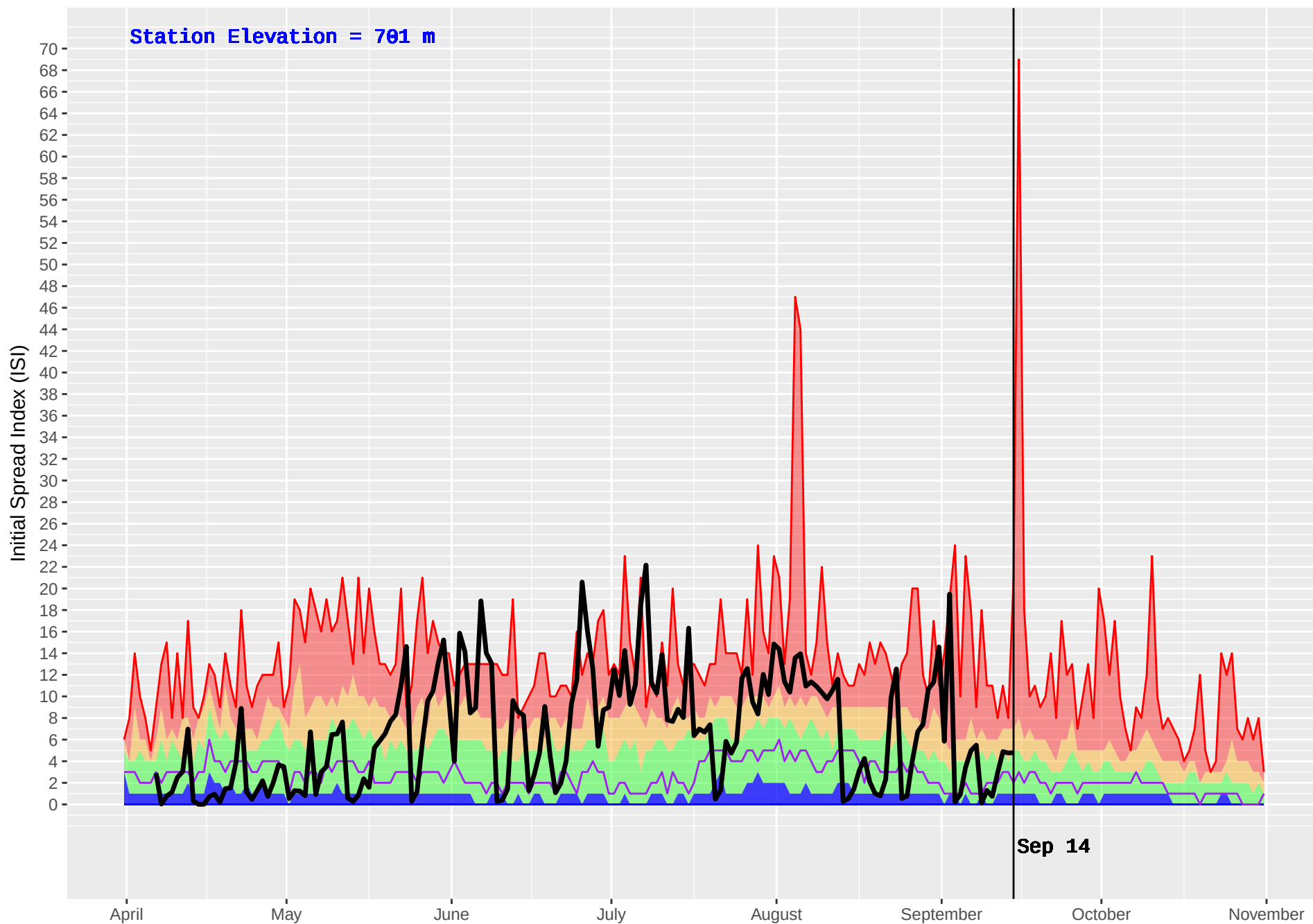
HORSEFLY (230) : Historical (1971–2016) and Current (2017) Noon Initial Spread Index (ISI)
